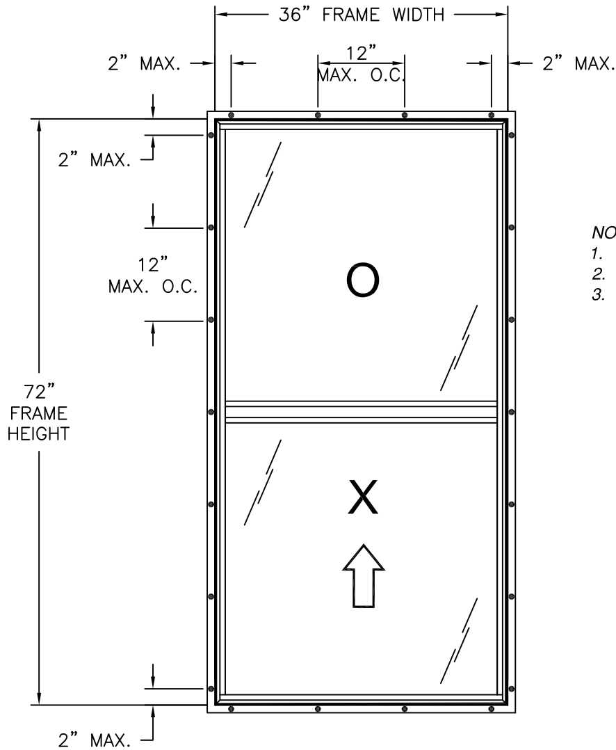
4000/4750 VINYL SINGLE HUNG TILT WINDOW EXTERIOR VIEW
