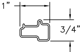
LOCK RAIL/ STILE REINFORCEMENT (11581) ALUMINUM 6063-T5
