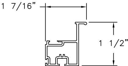
LIFT RAIL (4006) EXTRUDED RIGID PVC
