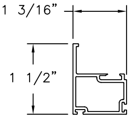
SASH STILE (4005) EXTRUDED RIGID PVC
